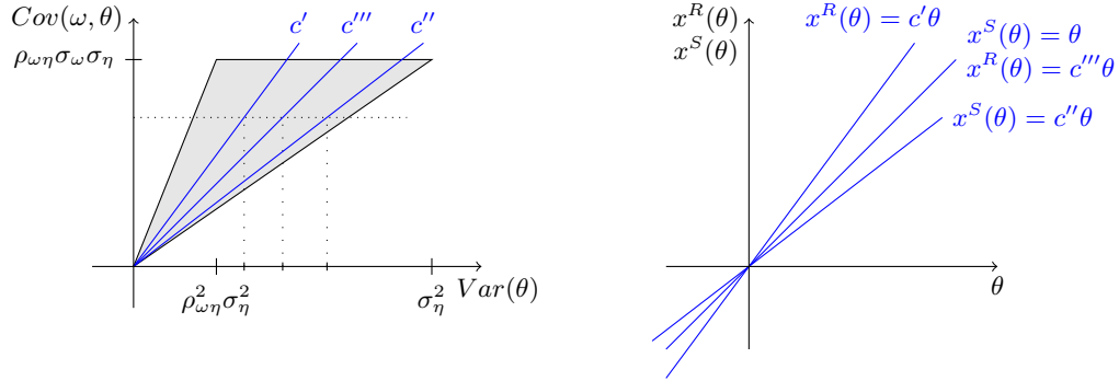
Figure 2: Conflict in terms of covariance and variance (left panel), and actions (right panel).
