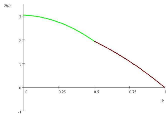
Figure 2: Joint Surplus for \lambda = 3 .
